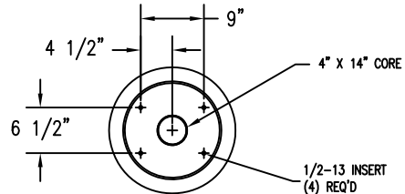
4 BOTTOM VIEW
