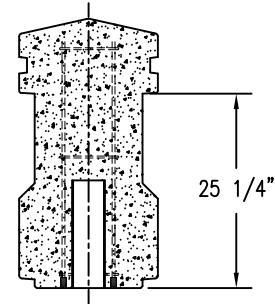
5 CROSS SECTION
