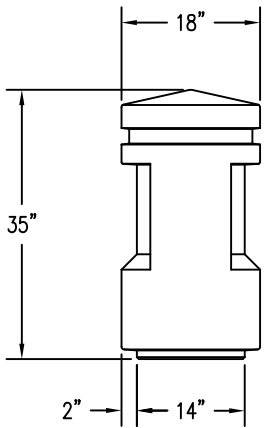
1 SIDE ELEVATION VIEW
